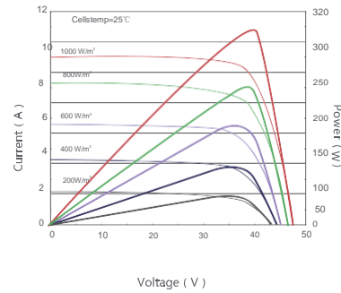
Current-Voltage & Power-Voltage Curves (315W)
